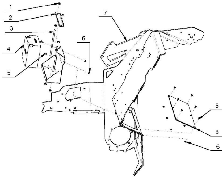
1.26.1 LAVINA® 30GKS7; 25GKS7 CARRIAGE 4 PARTS
