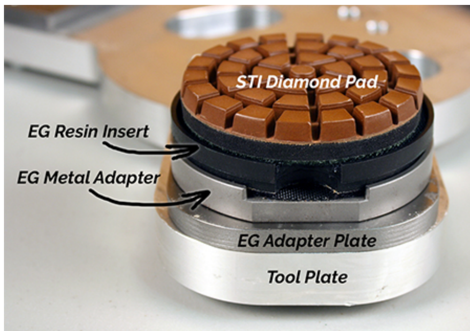
The "EG Resin Insert"
